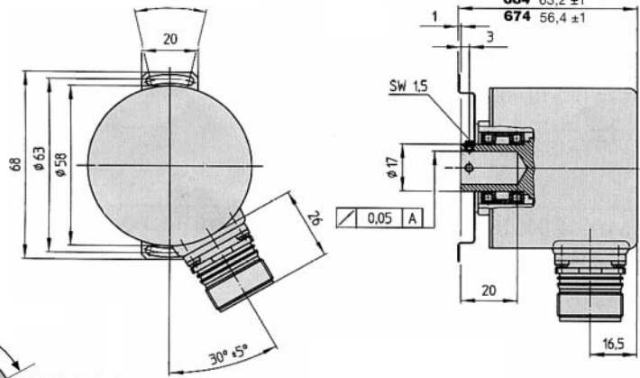
674 / 684 Hollow shaft
